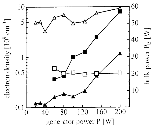
Fig. 5. Electron density n_e (□, △) and bulk power P_B (■, ▲) vs. on generator power P , in SF 6 (▲, △) and CF 4 (■, □) at 2 Pa, measured with SEERS.
