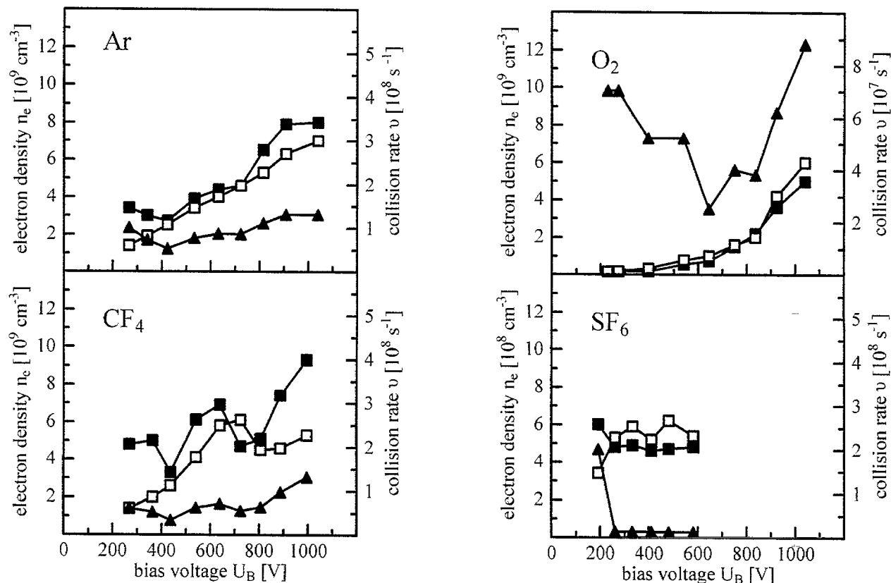
Fig. 4. Electron density n_e (■: SEERS; □: LP) and collision rate \nu (▲) vs. on bias voltage U_B in Ar, \text{CF}_4 , \text{O}_2 , and \text{SF}_6 at 2 Pa.
